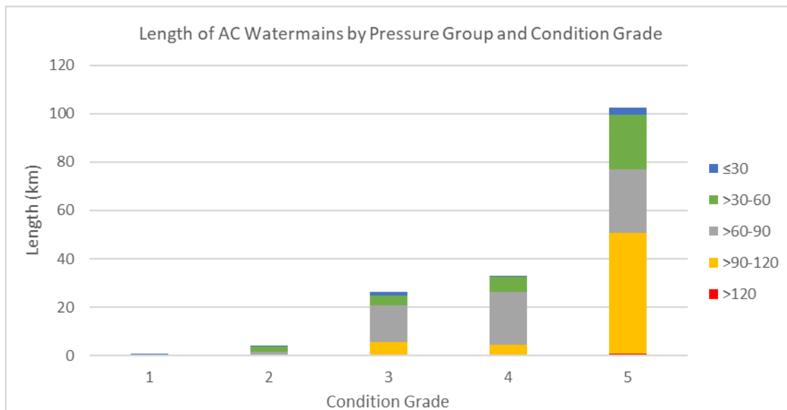
Graph 13 Length of AC watermain by Pressure Group and Condition Grade
