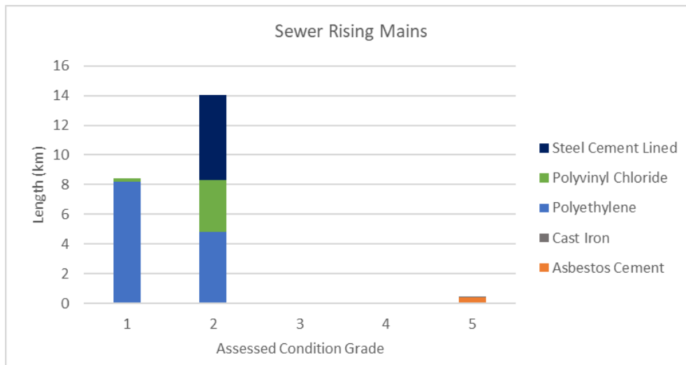
Graph 6 Wastewater Rising Mains: Total length of assets by material type and assessed Condition Grade
