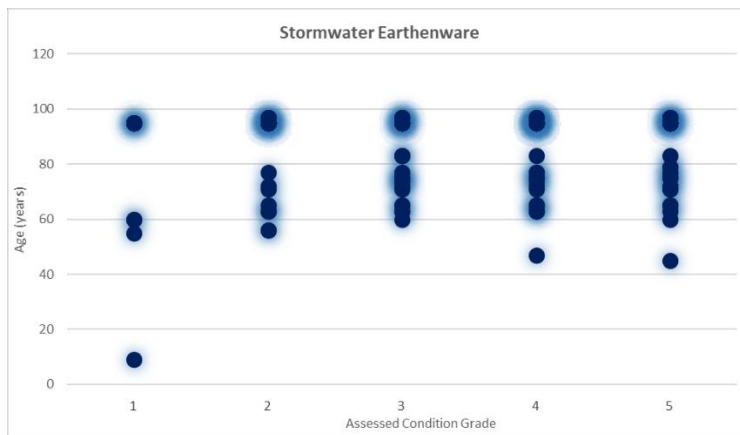
Graph 21 Stormwater Earthenware
