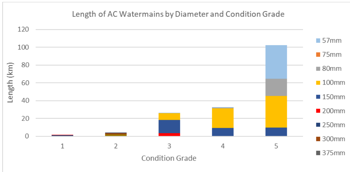
Graph 14 Length of AC watermain by Diameter and Condition Grade
